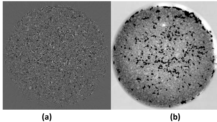
Gridrec reconstruction performed using the TOMCAT pipeline without (a) and with phase retrieval (1) (b)
