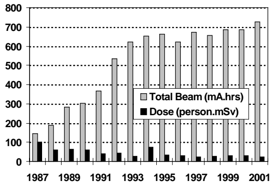
Figure 5. Collective dose rates
