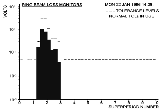
Figure 1. Prompt beam loss in the synchrotron
