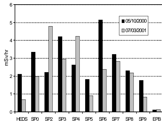
Figure 2. Average induced activity
