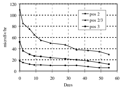
Figure 3. Induced radiation decay
